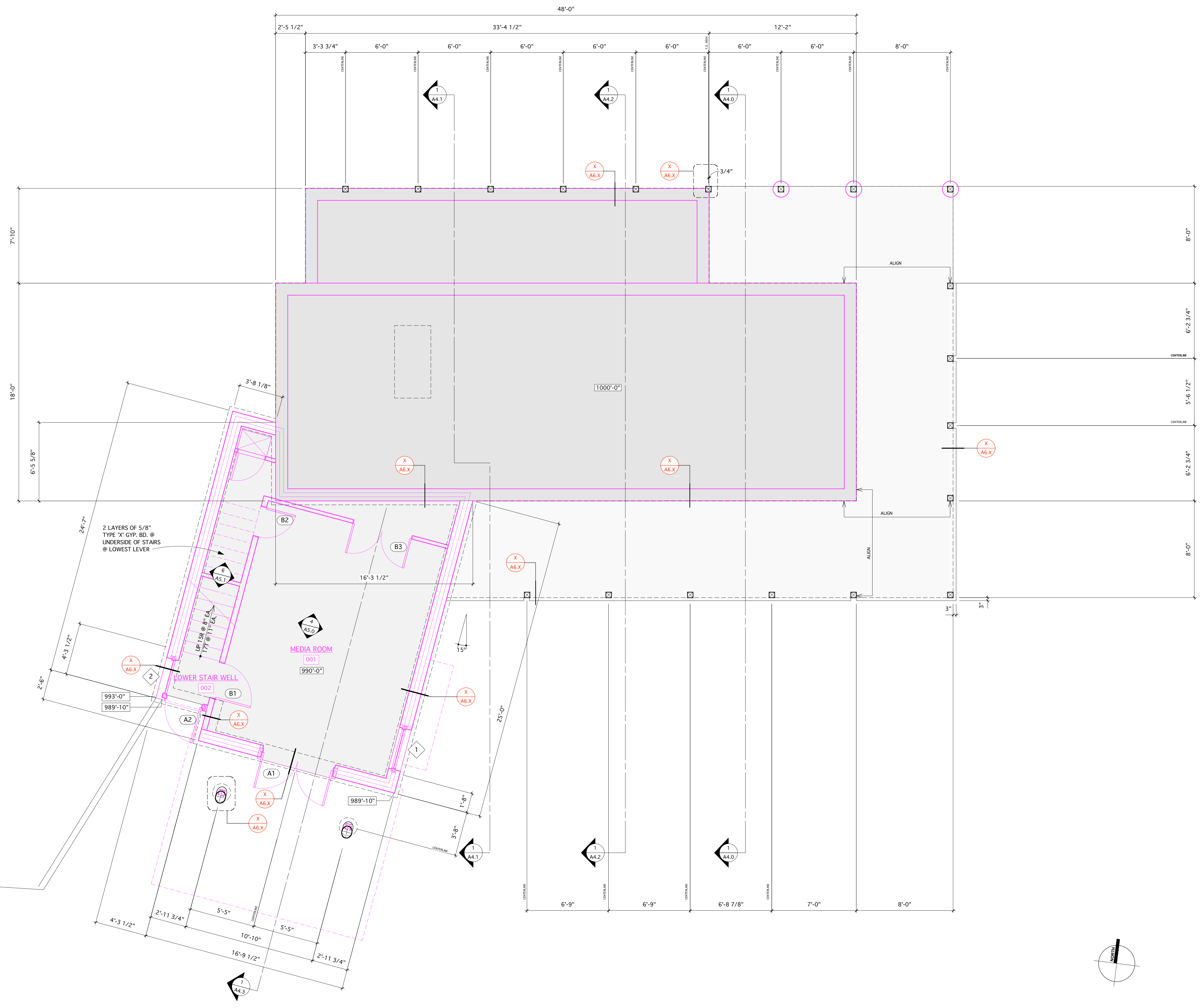
1 FLOOR PLAN - LOWER LEVEL A2.0 SCALE: 1/4" = 1'-0"
